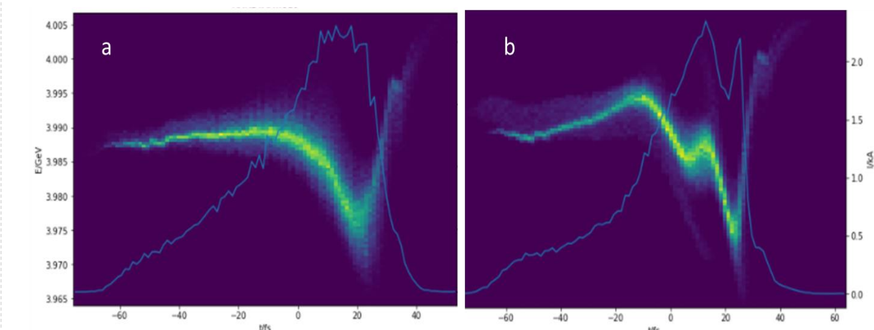
Figure 5: LCLS-II beam (a) before and (b) after laser shaping.
