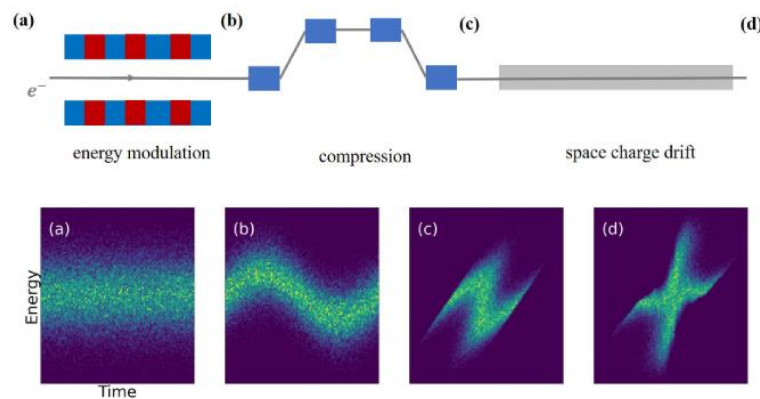
Figure 1: Physical System
