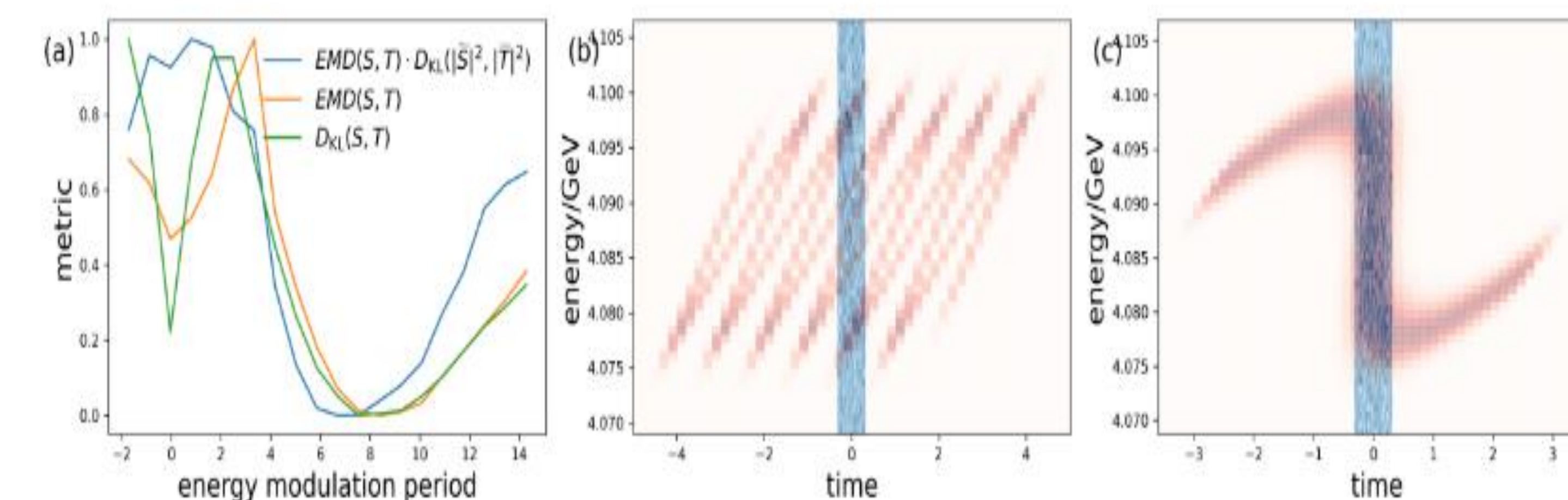
Figure 3: Combined Metrics to mitigate local minimum
