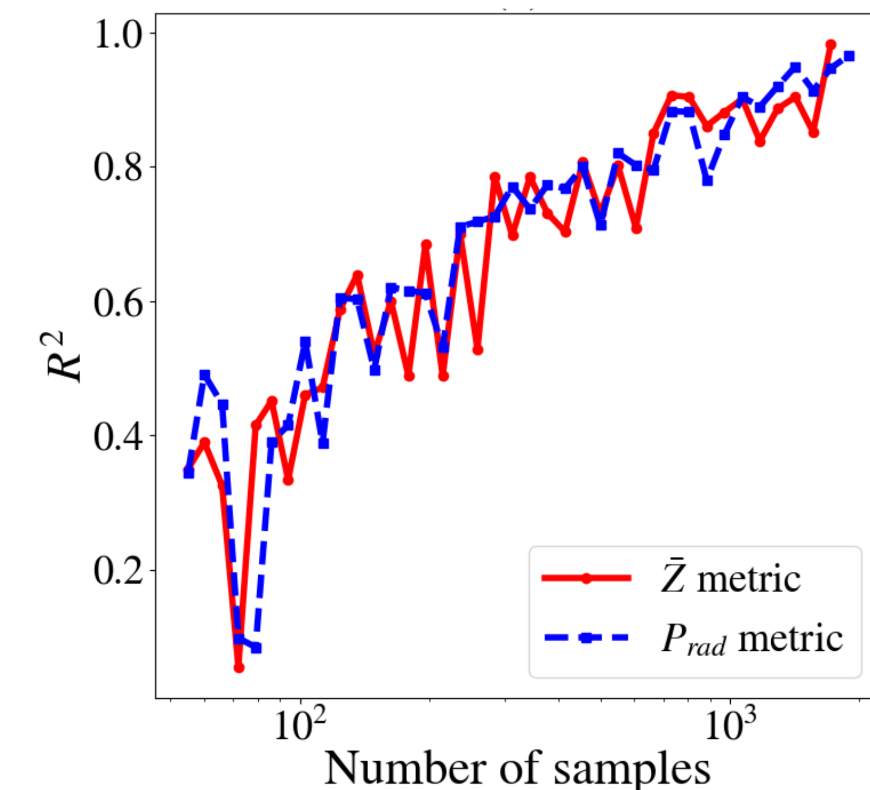
Figure 1. Validation R^2 improvement with acquired samples. The two curves are for separately trained surrogates using either average ion charge, or total radiation power as scalar metrics of the RFR surrogate.
