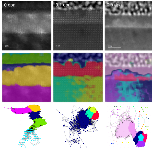
Figure 3: Cross-sectional STEM-HAADF images (top), segmentation maps (middle), and similarity graphs (bottom) for films irradiated to 0 (left), 0.1 (center), and 0.5 dpa (right).
