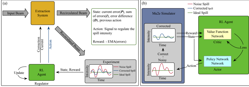
Figure 2: (a) : The Mu2e simulator initially generates the beam. It proceeds to adjust the spill and employs this adjusted spill to compute relevant information such as the state and reward. These pieces of information are instrumental in training the RL agent, which in turn offers new actions to refine the spill. (b) : The simulator refines (corrects) the spill derived from noisy data. It conveys the state and reward, calculated using the corrected spill, to update the value network responsible for evaluating the quality of the correction. Subsequently, the state and loss generated by the value network contribute to the adaptation of the policy network. The policy network, in response, generates new actions for spill regulation.
