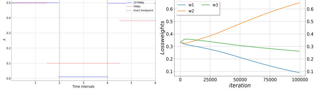
Figure 5: (Left) Parameter estimation of CP-PINNs and PINNs. (Right) Loss weights distribution across time.
